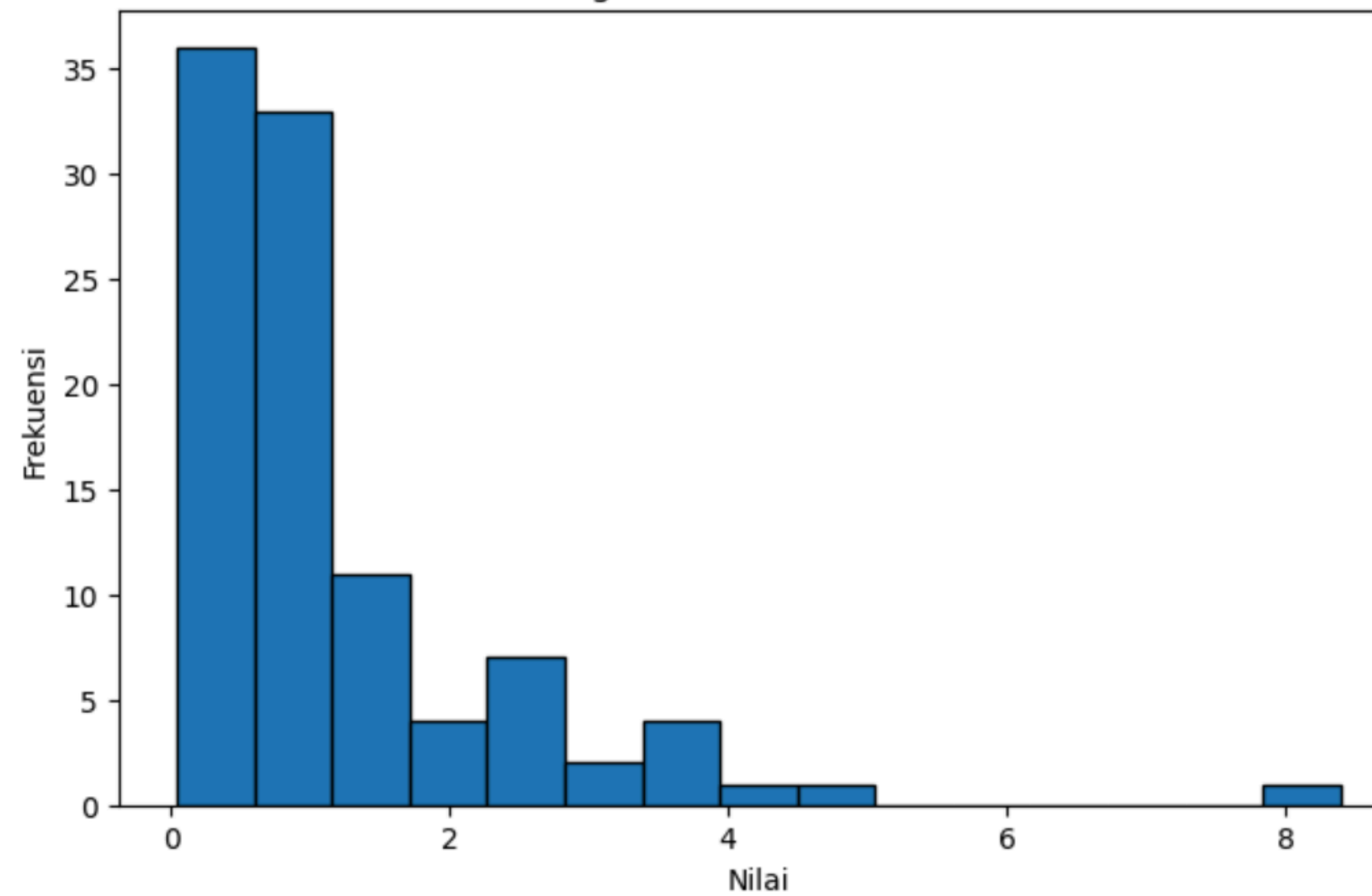
Histogram Data F-Distribution
